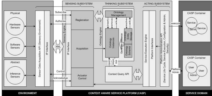
Figure 3. CASP Architecture.
